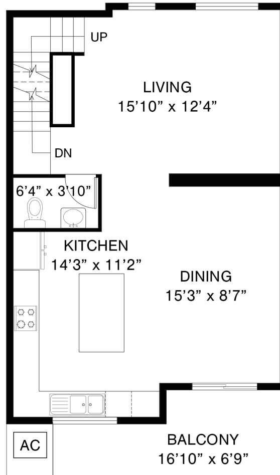
MAIN LEVEL 660 SQFT
