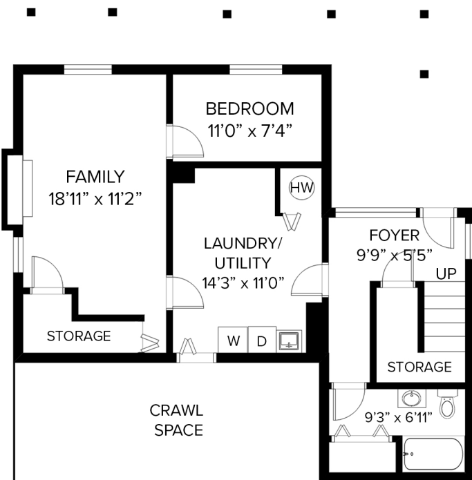
LOWER FLOOR 808 SQFT CEILING HEIGHT 7'3"
